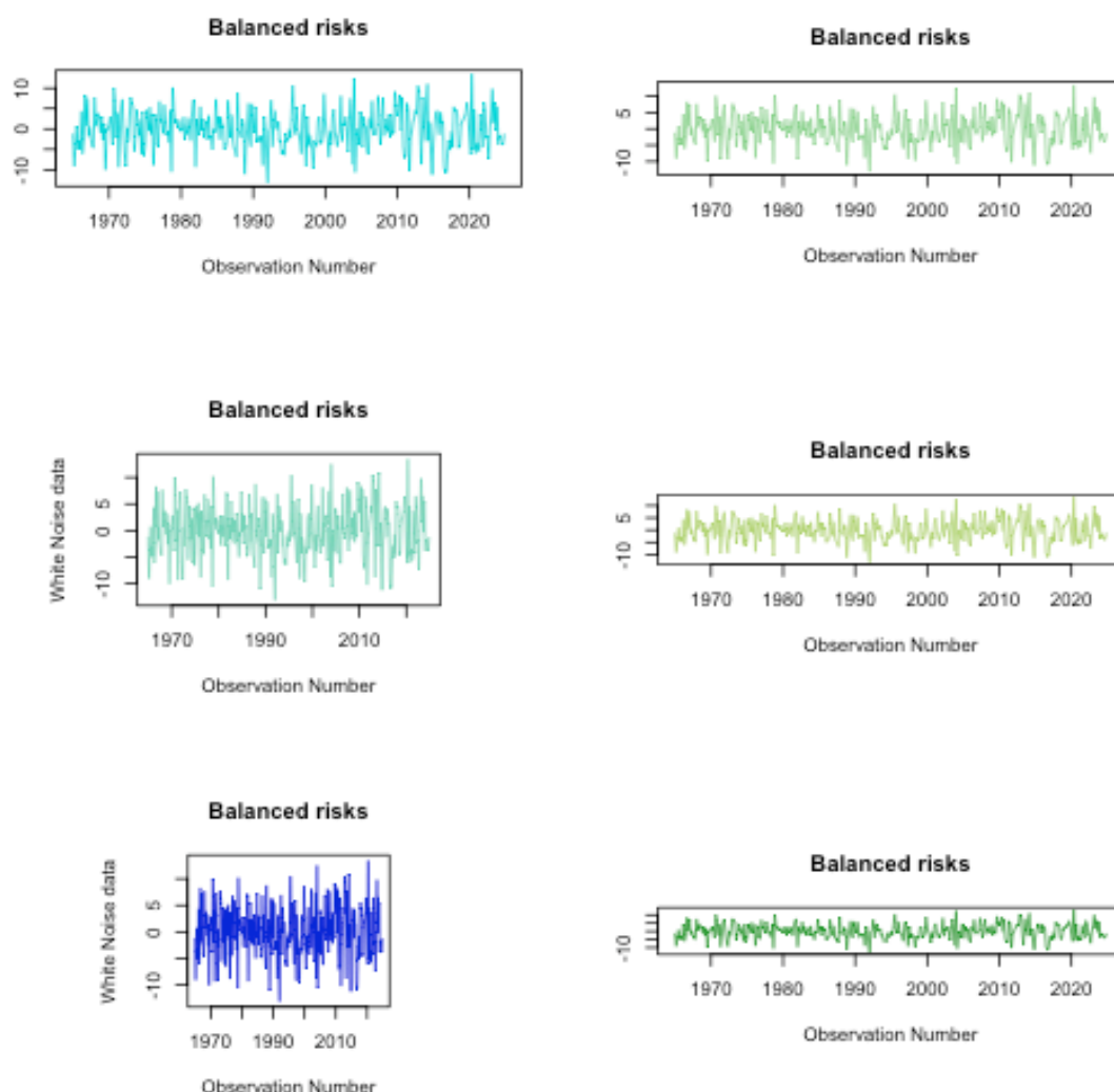
Figura 1.13: White noise
